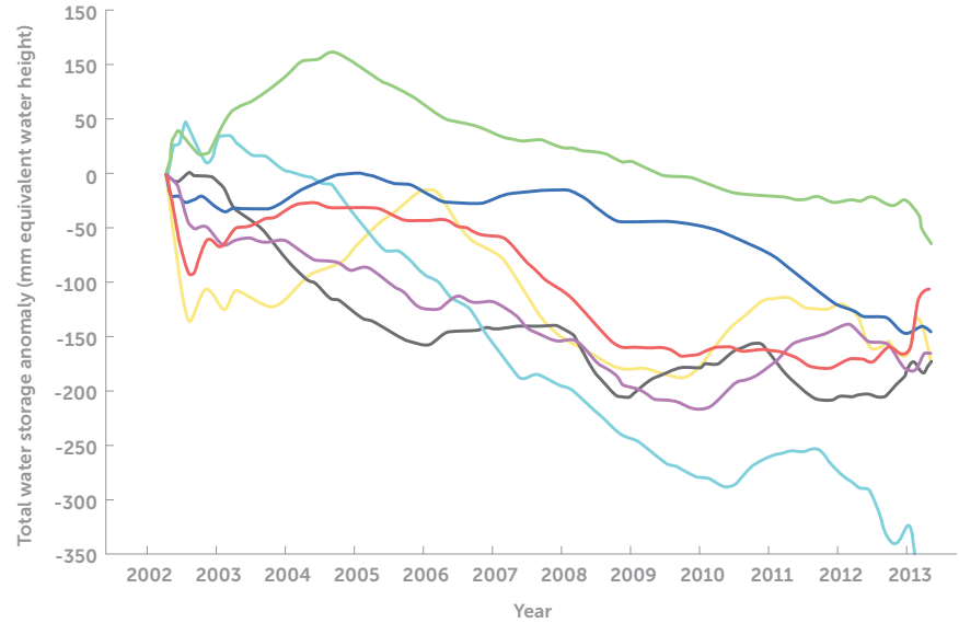
Water storage declines (mm equivalent water height)
